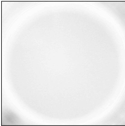
Stimulus: none ( 4 \times 10^4 cells/well)
