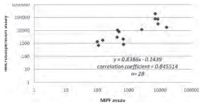
Fig. 1. Correlation of the potencies expressed in log of number of revertants per µg of EOM or mL equivalent obtained in the MPF assay and in the microsuspension Salmonella/microsome assay for the samples tested using TA98 with and without S9.
